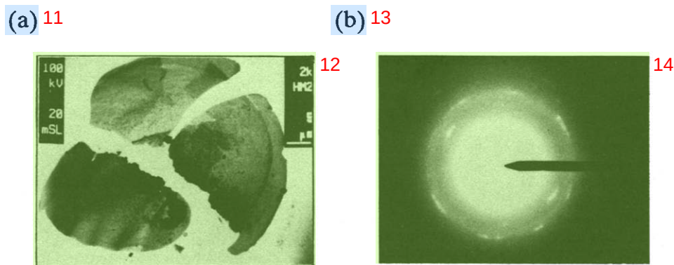
Fig. 7. Transmission electron microscopy of an extracted pit cover: (a) Bright field micrograph of cover fragments; (b) Selected area electron diffraction pattern.
