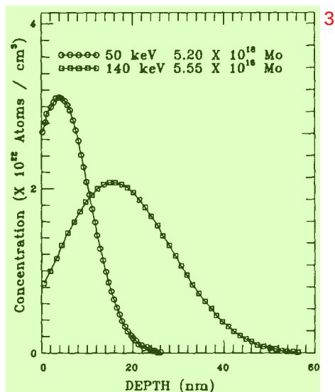
Fig. 2. Distribution of molybdenum within the implanted alloy, comparing the same dose for different implanting energies.
