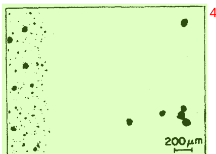
Fig. 8. Optical micrograph of sample half-implanted with krypton and anodically polarized identically to the sample of Fig. 5(a).
