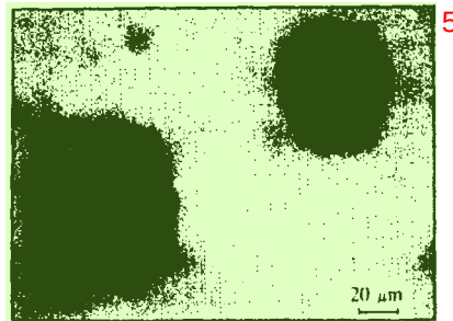
Fig. 12. Optical micrograph of curled-up covers from pits on a sample similar to that shown in Figs. 5(a) and 9(a).
