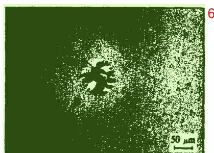
Fig. 10. Nomarski interference contrast in optical micrograph of a typical pit on implanted steel surface.
